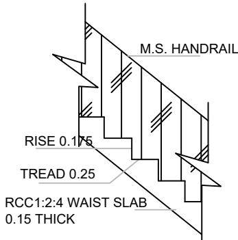
STAIRCASE DETAILS SCALE- 1:50
