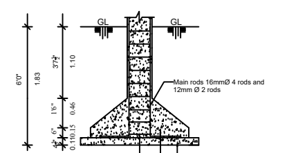
SECTION ON - FF
