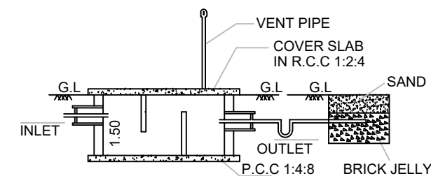
SECTION-AB
