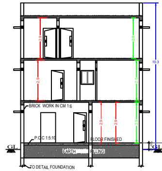
SECTION "A-B"
