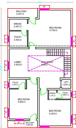
PRO.SECOND FLOOR PLAN SCALE:1:100
