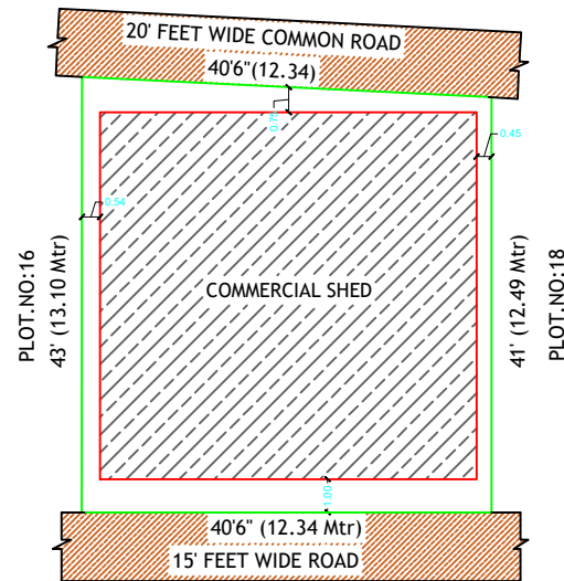
SITE PLAN
