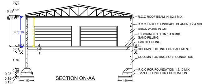
SECTION ON-AA
