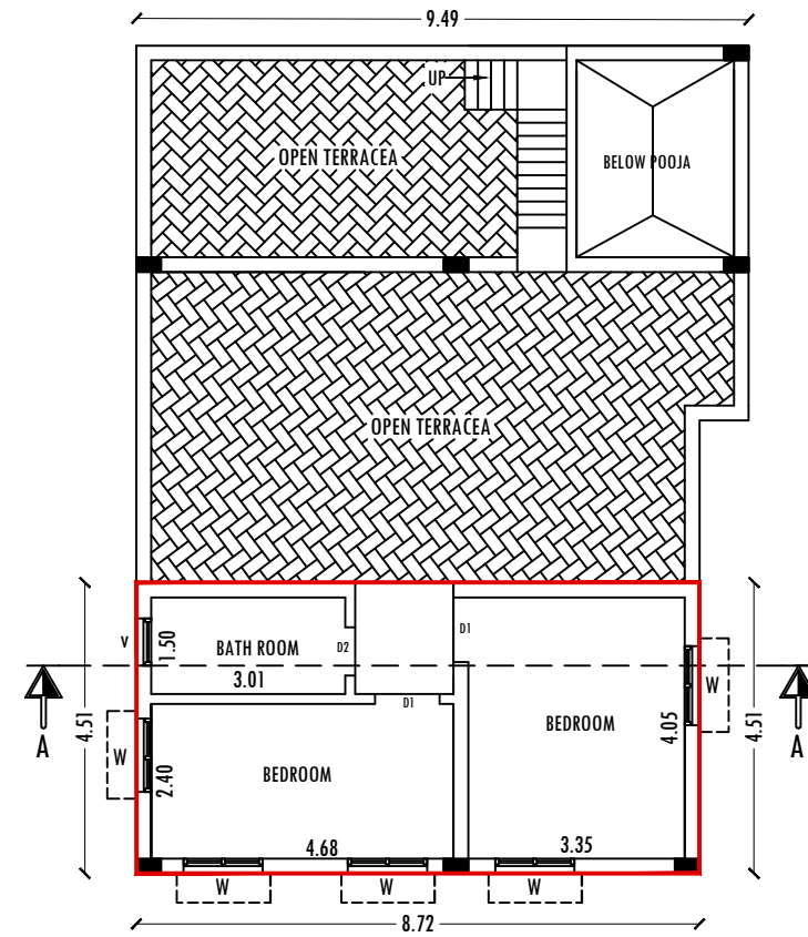
PRO-SECOND FLOOR PLAN
