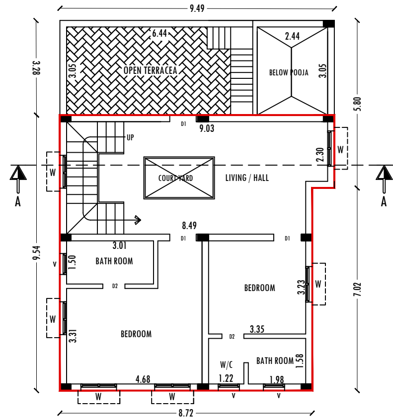
EXTG-FIRST FLOOR PLAN
