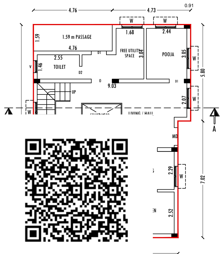
EXTG-GROUND FLOOR PLAN
