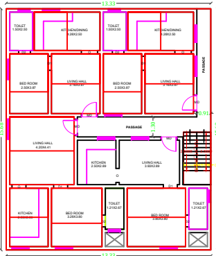
PRO. FIRST FLOOR PLAN.
