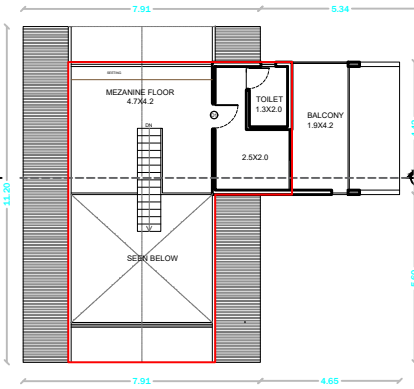
PRO.SECOND FLOOR PLAN SCALE:1:100
