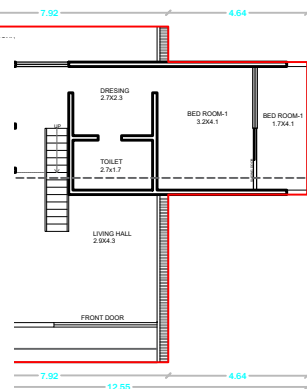
PRO.FIRST FLOOR PLAN SCALE:1:100
