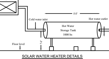
SOLAR WATER HEATER DETAILS
