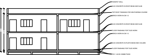
CROSS SECTION
