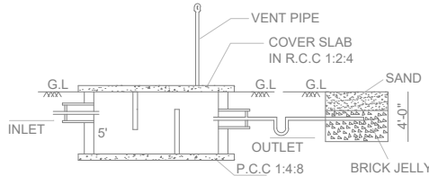
SECTION-AB
