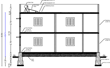
SECTION AT 'AA'
