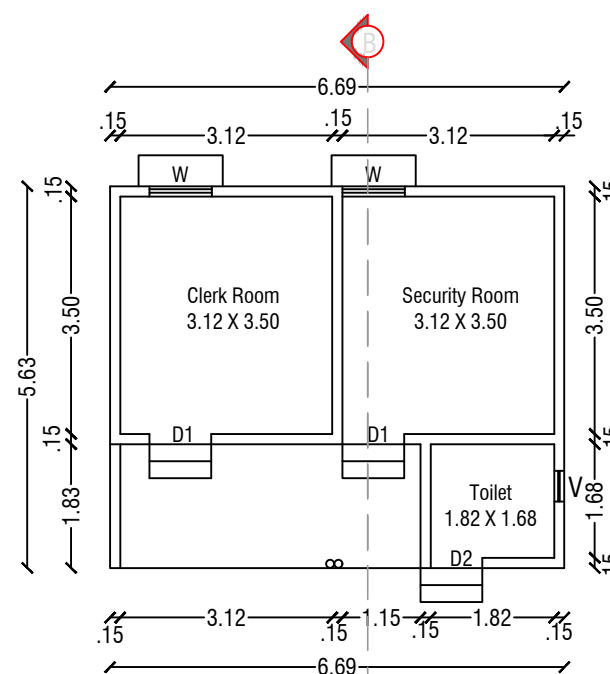
SECURITY & CLERK ROOM PLAN (Block - 2)
