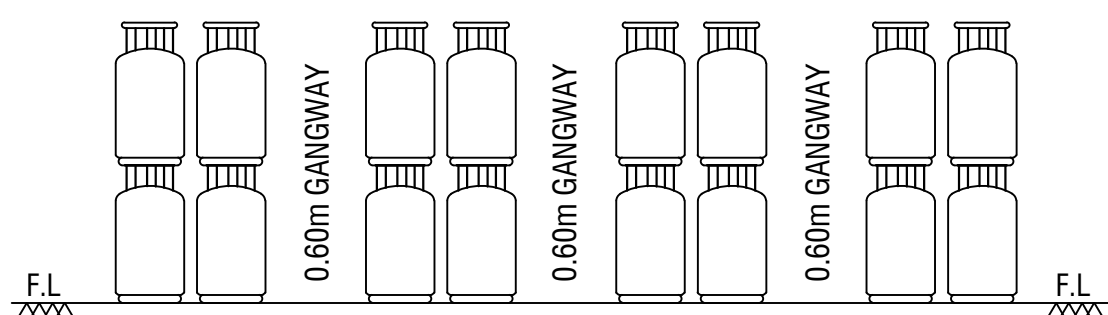
SECTIONAL ELEVATION OF STORAGE LPG CYLINDERS
