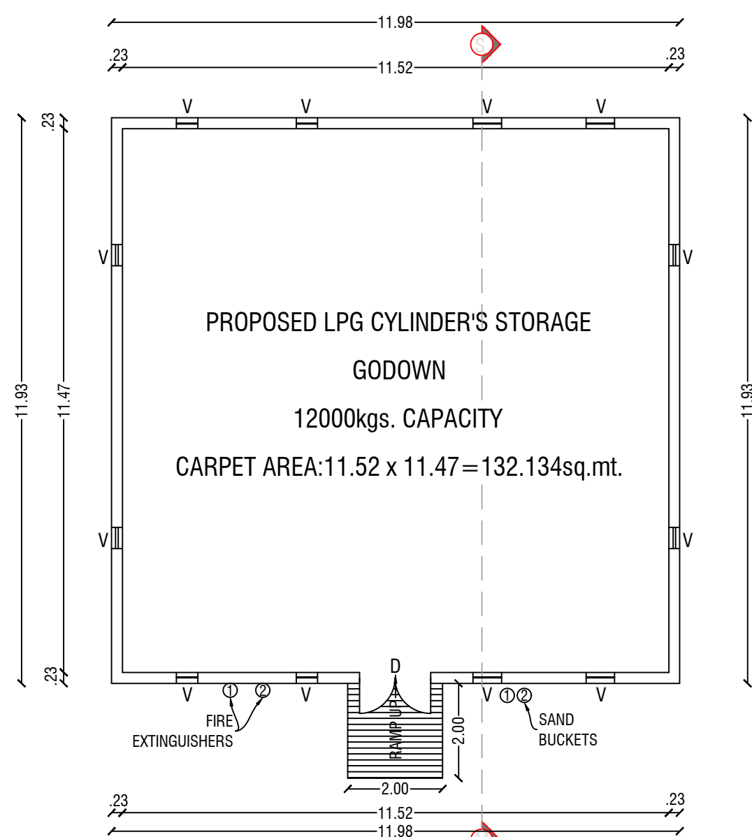
STORAGE GODOWN FLOOR PLAN (Block - 1)
