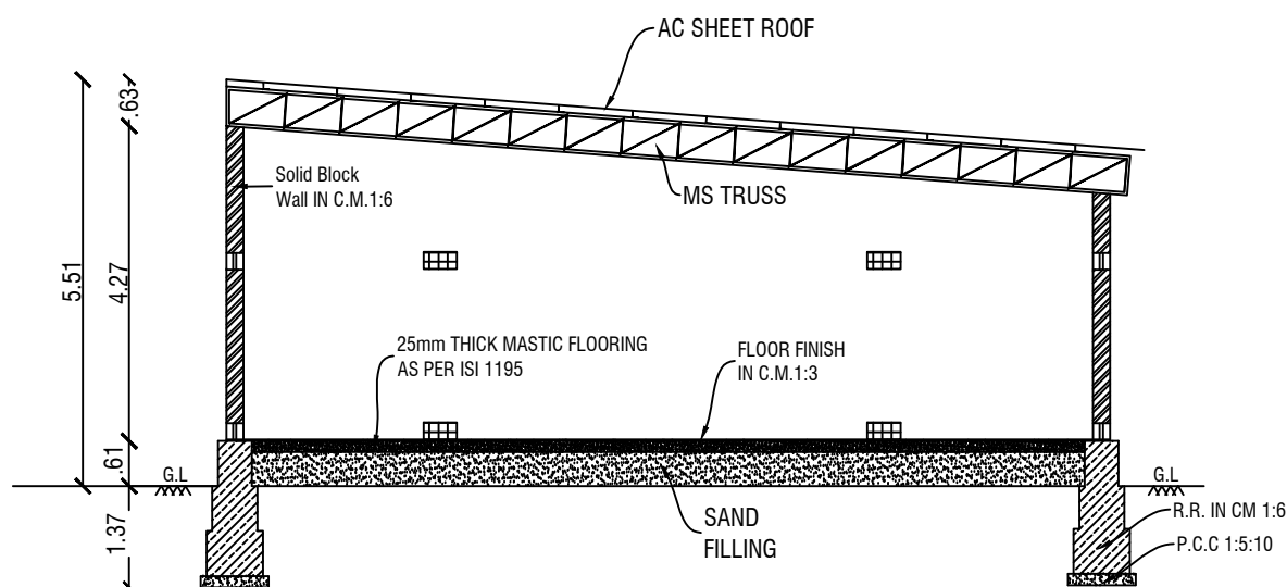
SECTION -SM
