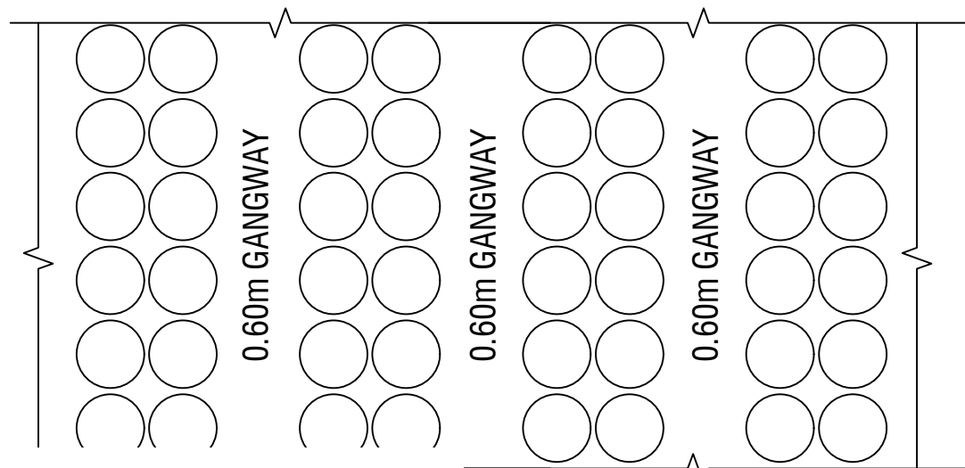
STORAGE PLAN
