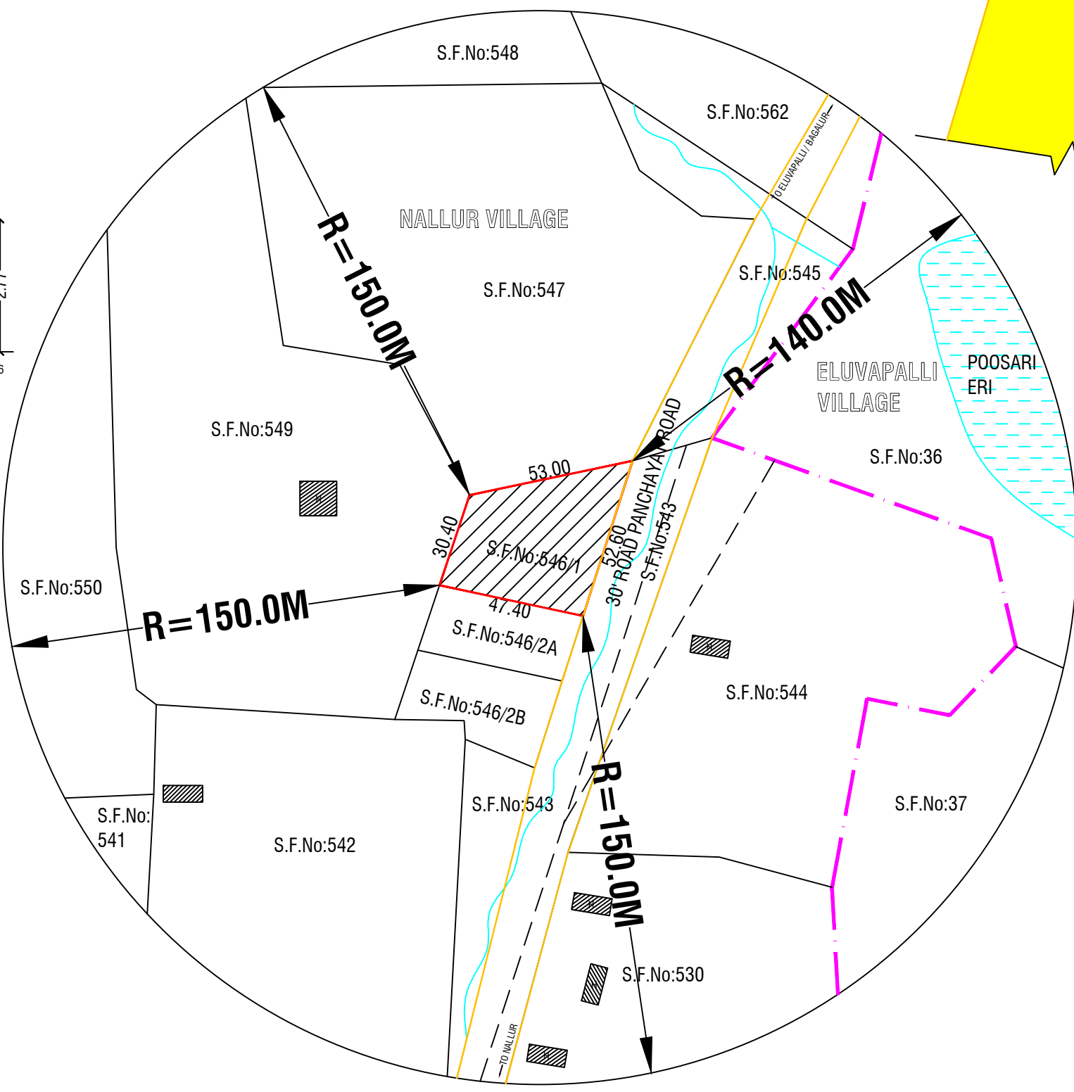
TOPO PLAN SCALE 1:1600
