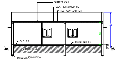
SECTION "A-B"
