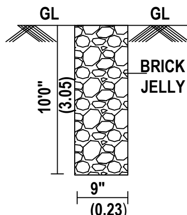
PERCOLATION PIT
