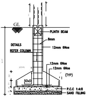
FOUNDATION DETAILS
