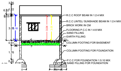
SECTION ROOMS
