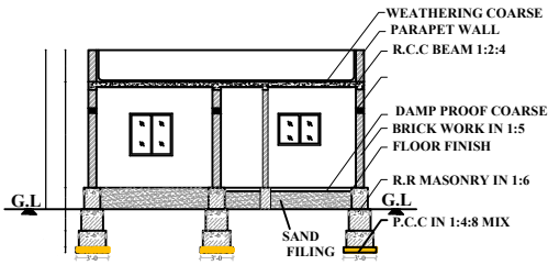
SECTION KITCHEN
