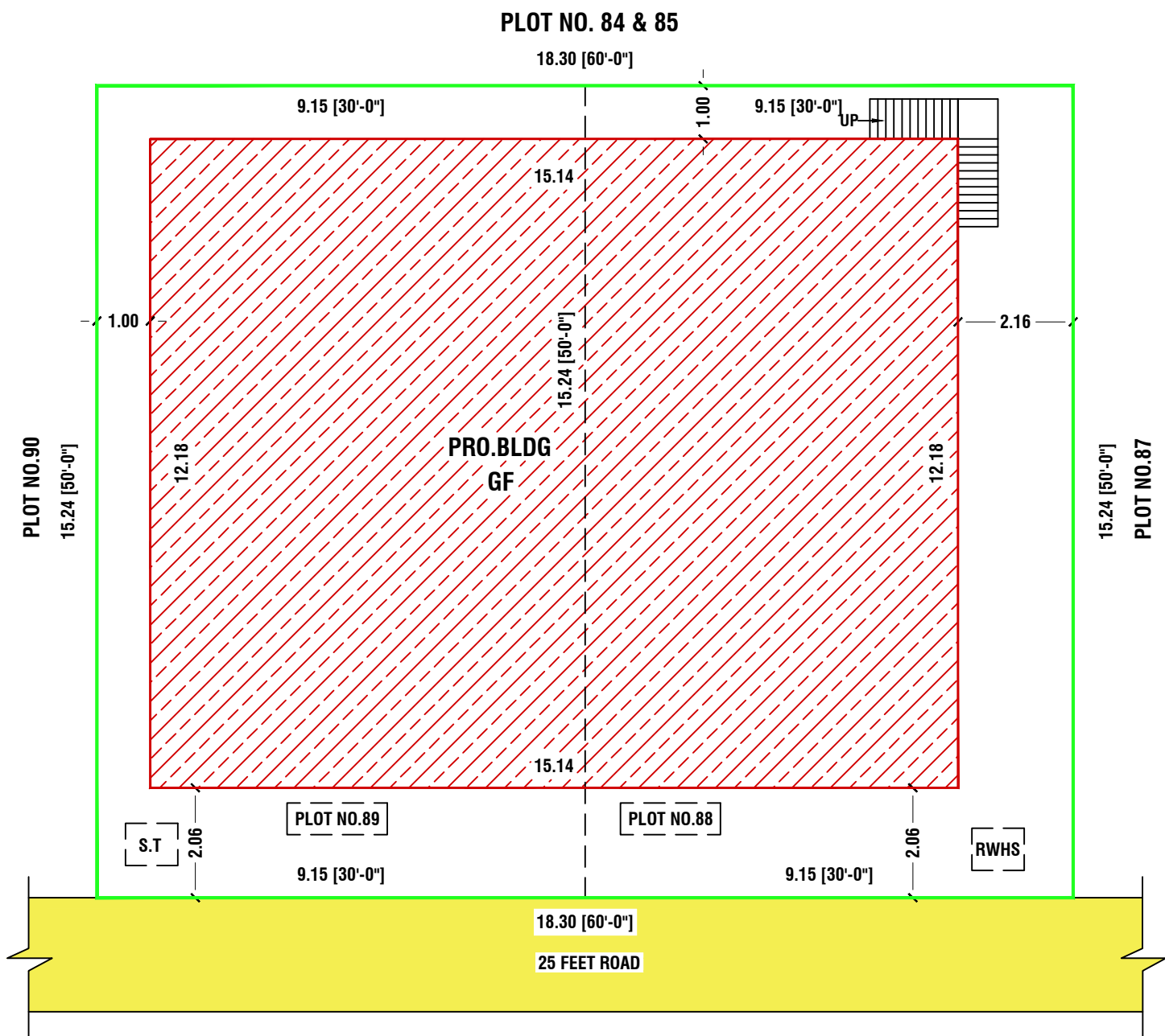
SITE PLAN
