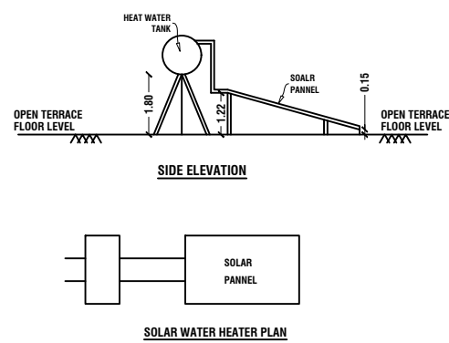
SOLAR WATER HEATER PLAN
