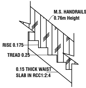
STAIRCASE DETAILS
