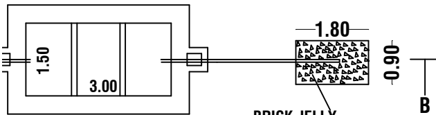
TIC TANK & DISPERSION TRENCH DETAILS
