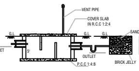
SECTION-AB
