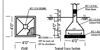
FOOTING DETAILS
