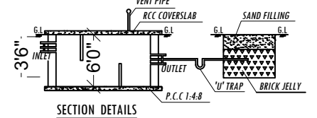
SEPTIC TANK AND DISPERSION TRENCH DETAILS
