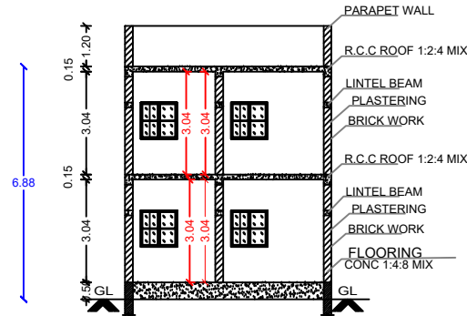
SECTION: A-B
