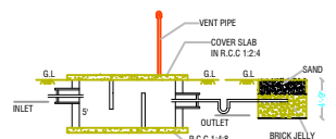
SECTION: A-B
