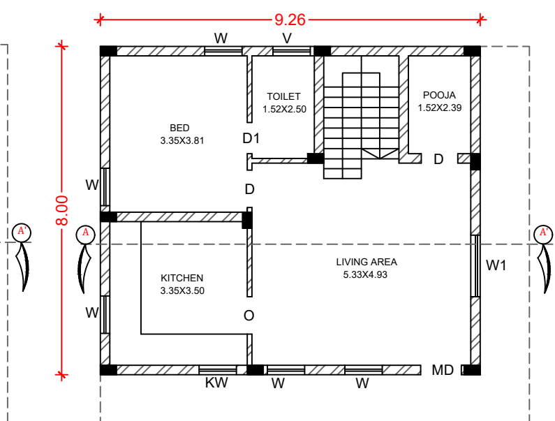
GROUND FLOOR (BLOCK -2)
