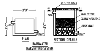
RAINWATER HARVESTING SYSTEM
