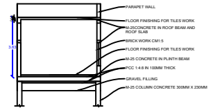
CROSS SECTION
