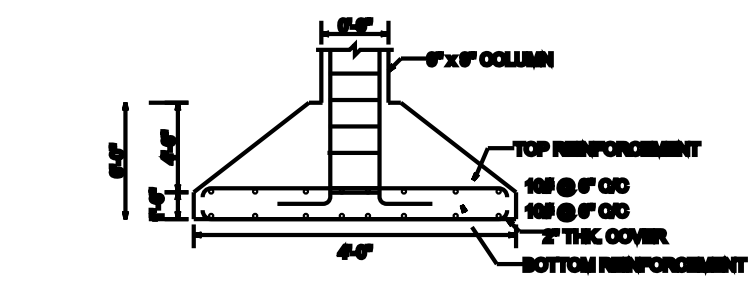
TYPICAL FOOTING
