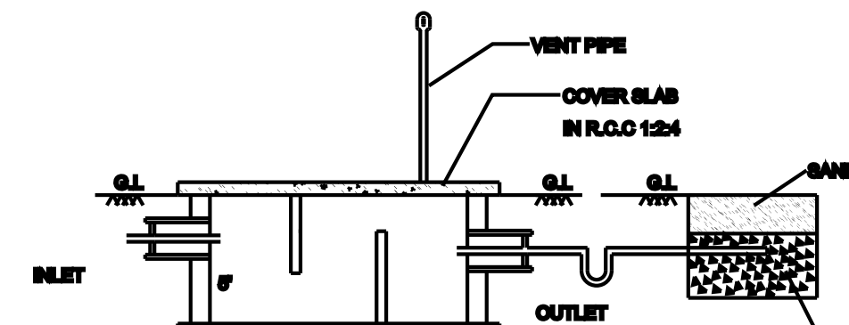
SECTION-AB
