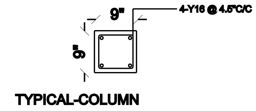
TYPICAL COLUMN
