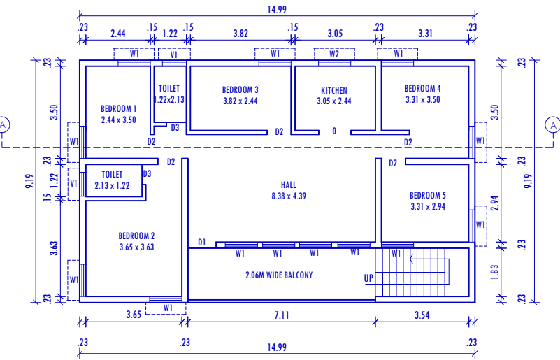
TYPICAL FIRST & SECOND FLOOR PLAN
