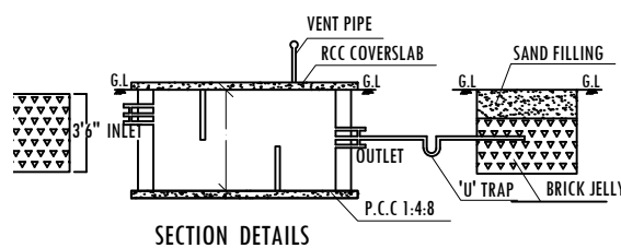
SECTION DETAILS SEPTIC TANK AND DISPERSION TRENCH DETAILS
