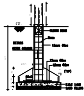
FOUNDATION DETAILS
