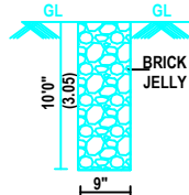
PERCOLATION PIT
