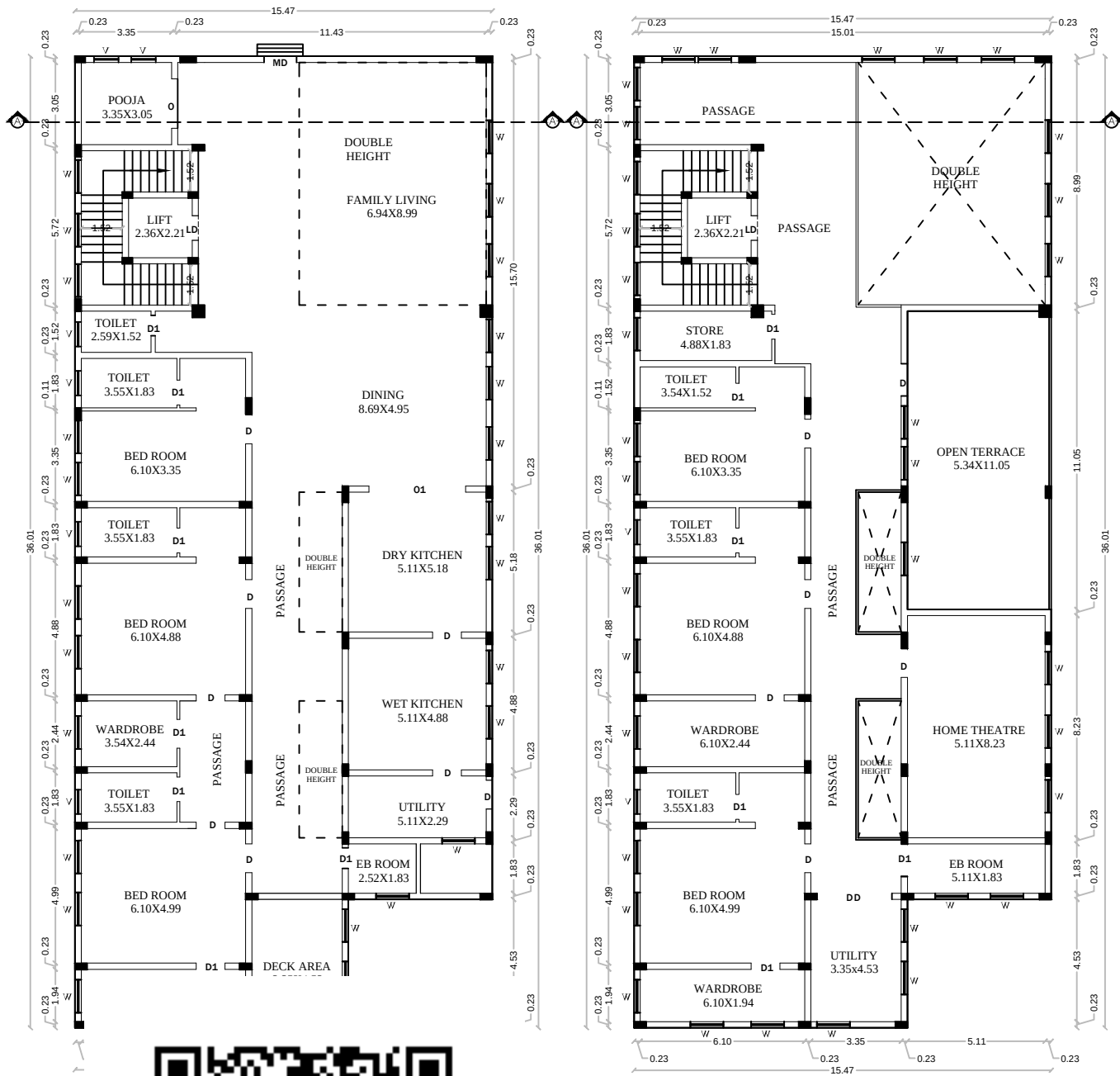
FIRST FLOOR SCALE - 1:100
