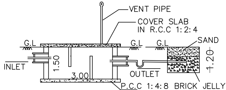
SECTION-AB
