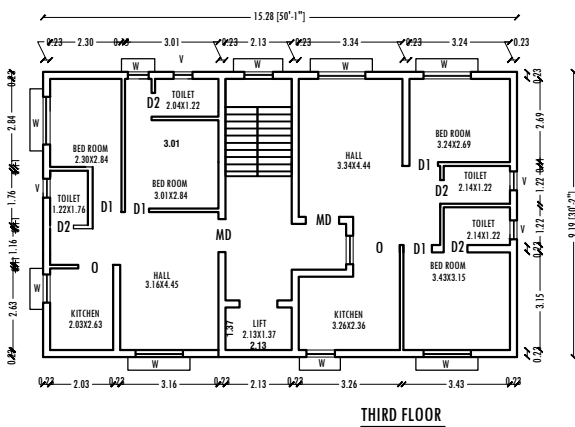
THIRD FLOOR
