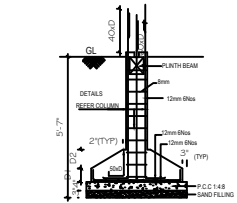
FOUNDATION DETAILS SCALE : 1:50
