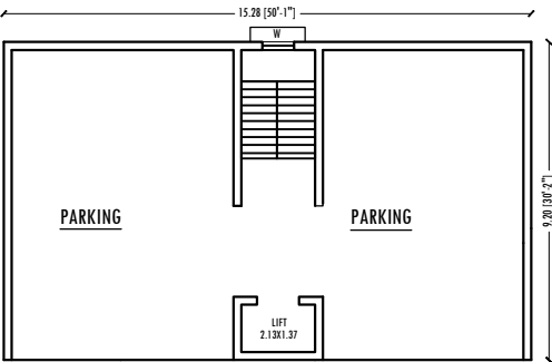
STILT FLOOR
