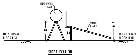
SIDE ELEVATION
