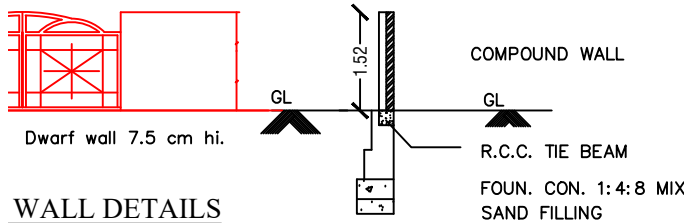
WALL DETAILS
