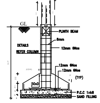
FOUNDATION DETAILS
