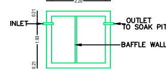
PLAN SEPTIC. TANK
