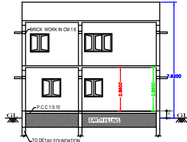
SECTION "A-B"
