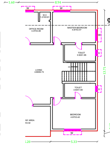
PRO.FIRST FLOOR PLAN SCALE:1:100
