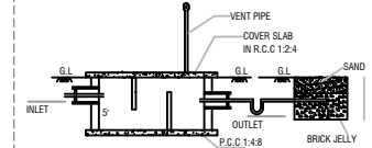
SECTION-AB
