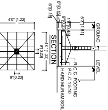
FOUNDATION DETAIL'S
