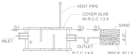
SECTION-AB
