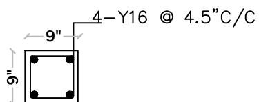
TYPICAL-COLUMN
