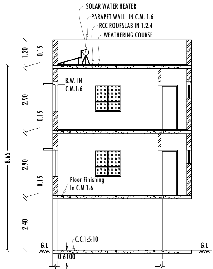
SECTION-AA
