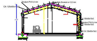
CROSS SECTION
