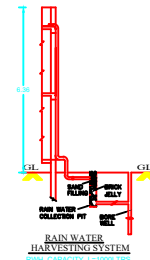
RAIN WATER HARVESTING SYSTEM RWHP_CAPACITY_L=1000LITRES
