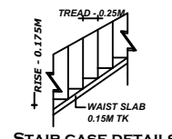
STAIR CASE DETAILS SCALE : 1:50
