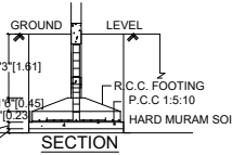
FOUNDATION DETAILS
