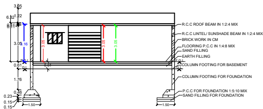
SECTION ON-AA
