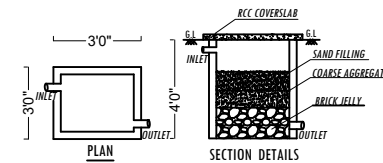
PLAN RAINWATER HARVESTING SYSTEM
