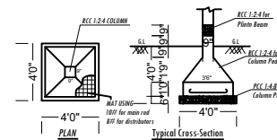
FOOTING DETAIL
