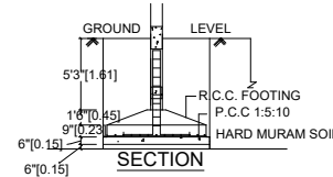
FOUNDATION DETAILS
