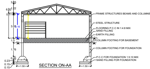
SECTION ON-AA
