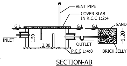
SECTION-AB
