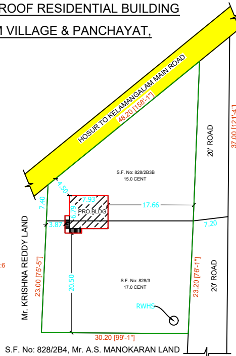
SITE PLAN
