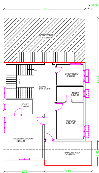
PRO.FIRST FLOOR PLAN SCALE:1:100
