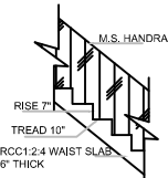
STAIRCASE DETAILS SCALE- 1:20
