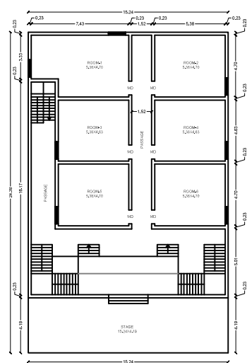
ALREADY APPROVED & REVISION FIRST FLOOR PLAN
