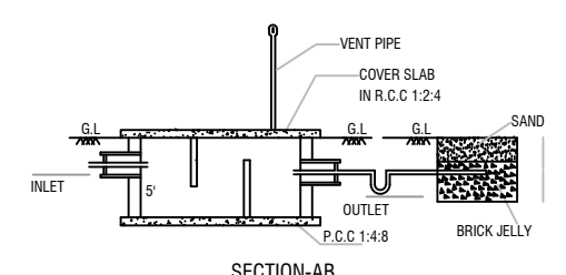
SECTION-AB
