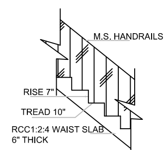
STAIRCASE DETAILS SCALE- 1:20
