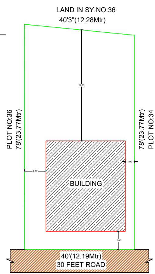
SITE PLAN SCALE:1:100 SITE PLAN
