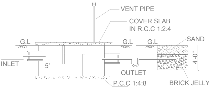
SECTION-AB
