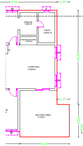
RST FLOOR PLAN SCALE:1:100
