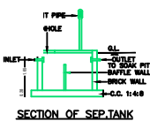
SECTION OF SEP.TANK
