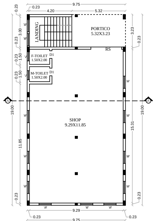
GROUND FLOOR SCALE - 1:100
