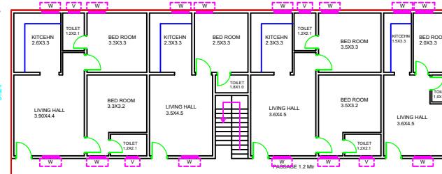
PRO.FIRST FLOOR PLAN
