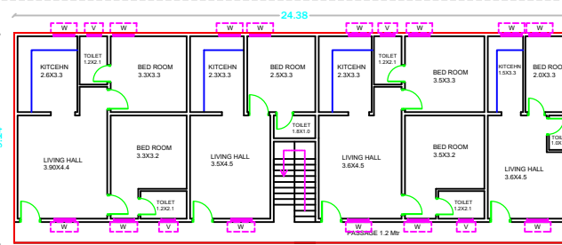
PRO.SECOND FLOOR PLAN
