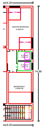
PRO. FIRST FLOOR PLAN.
